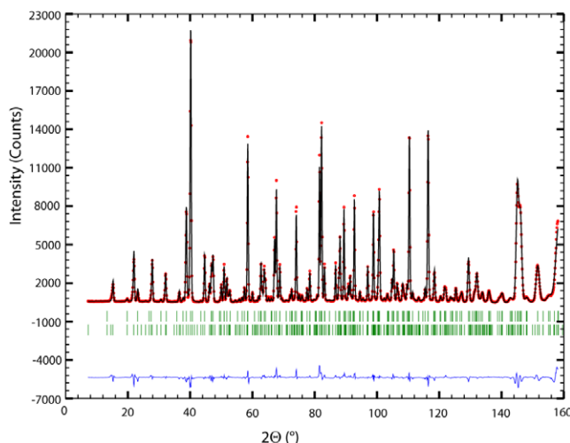
Figure 2. Observed (dots, red), calculated (line, black) and difference pattern of \text{YFe}_3(\text{BO}_3)_4 at 2 K refined in P3_121 . The tick marks indicate the calculated position of the nuclear (upper row) and magnetic (lower row) Bragg peaks.
