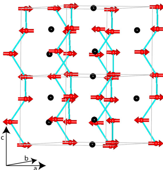
Figure 3. Magnetic structure of \text{YFe}_3(\text{BO}_3)_4 . Fe spins in red (grey), while the direct Fe-Fe exchange along the helicoidal chains is indicated by blue (light grey) lines. The position of the Y atoms is indicated by black spheres.
